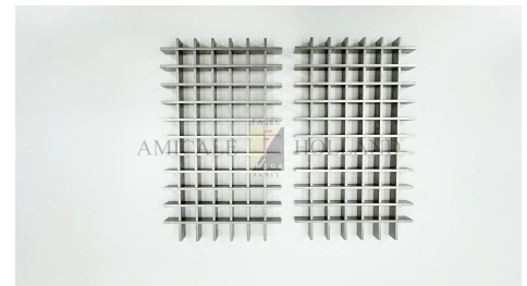
SET (2) CENTRE PARTS FOR SIDE GRILLES FVS/ HK IN ALUMINIUM STILL TO BE ANODISED
